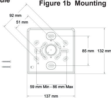
Figure 1b Mounting
