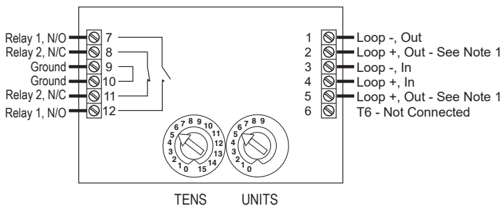
Figure 2: Module Wiring
