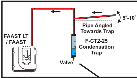
Figure 1: Typical example for set up
