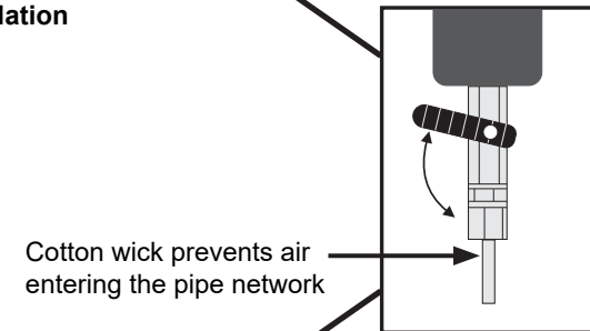
Figure 2: Valve Assembly - Closed Position
