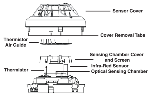
Figure 2: Cleaning the Sensor
