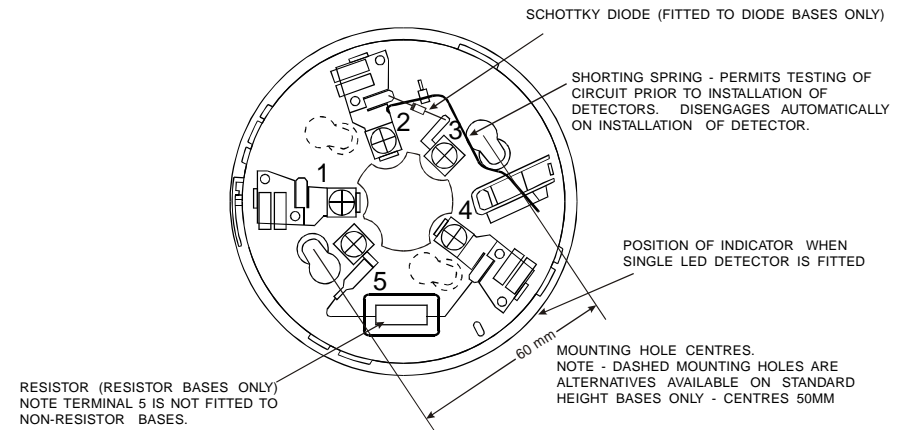
Figure 1: Terminal Layout
