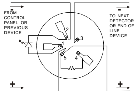
Figure 2b: Resistor Base Wiring
